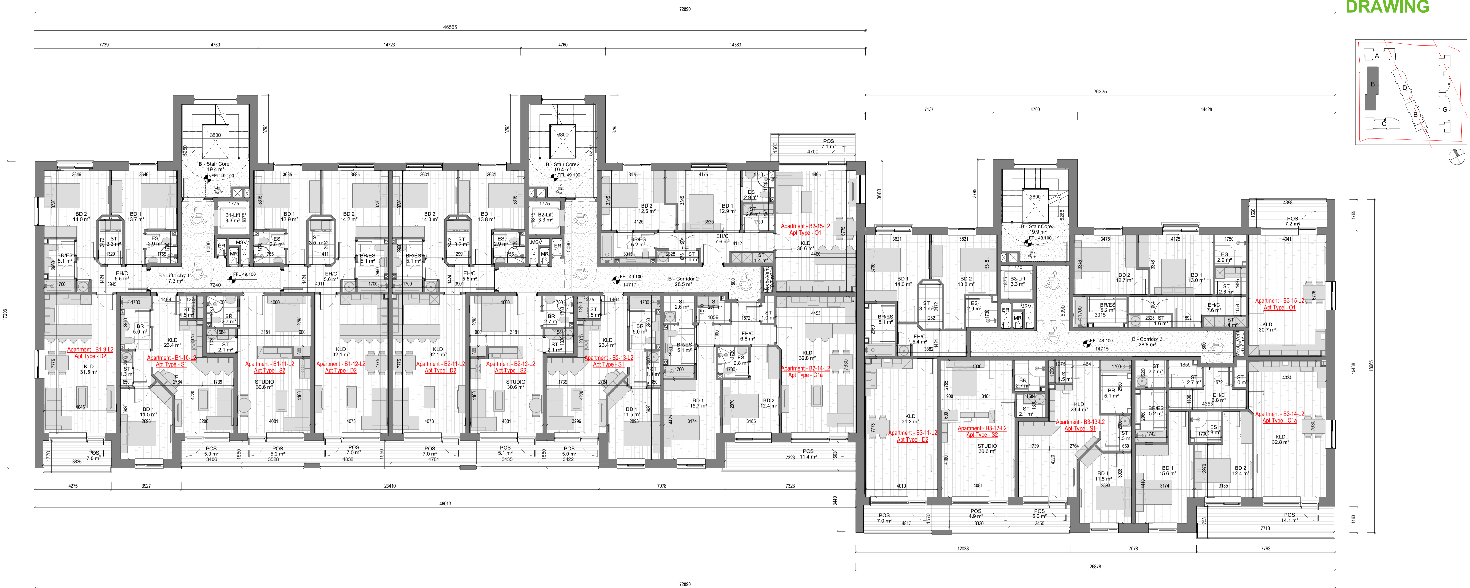
1 GA - Second Floor Plan 1 : 100
